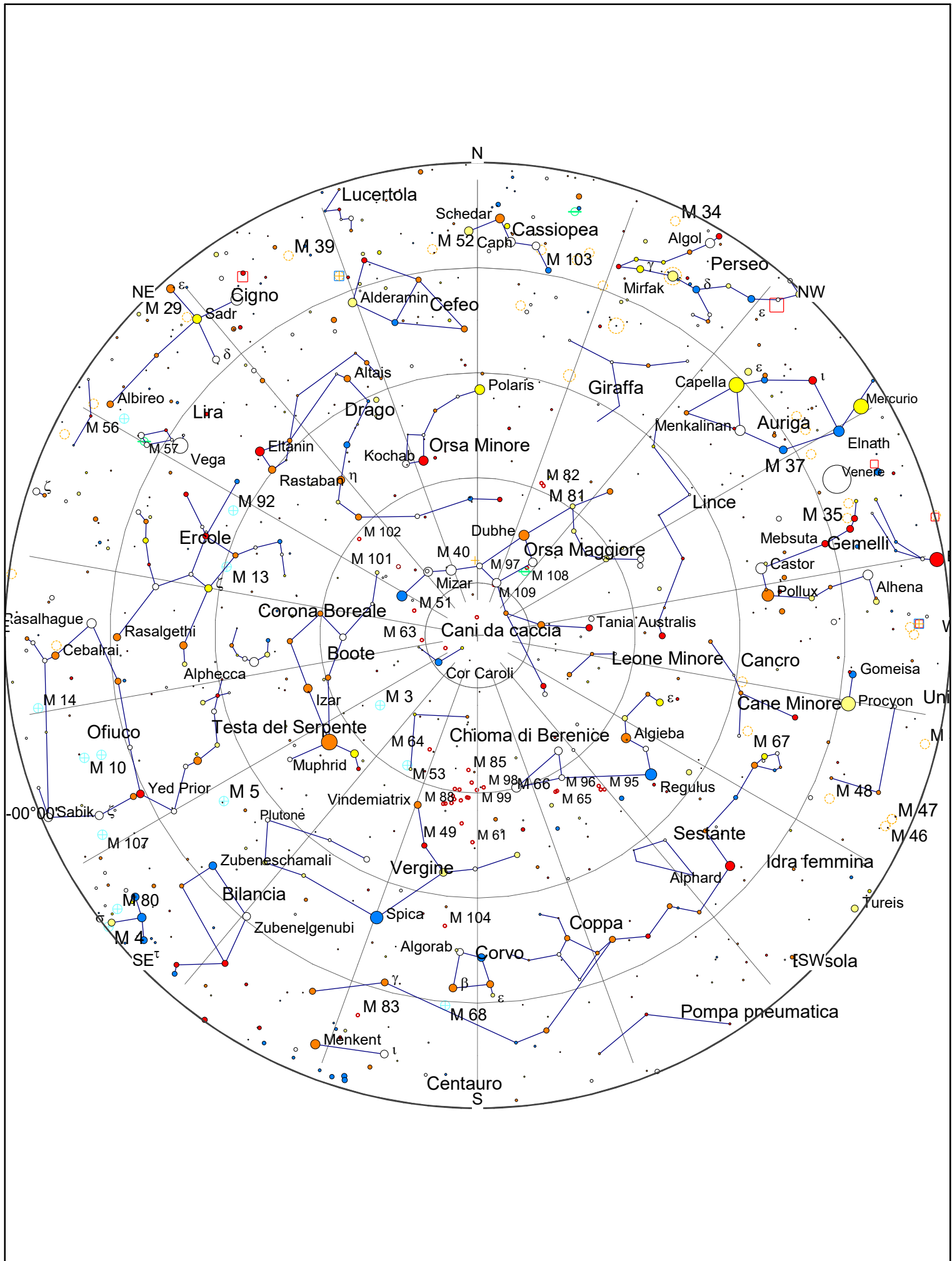
Coord. Alt/AZ ARC, Apparenti, Pescia, 1988-05-15, 22h00m00s (CEST), Mag:5.1/6.0,30.0', FOV:+180°00'01"
